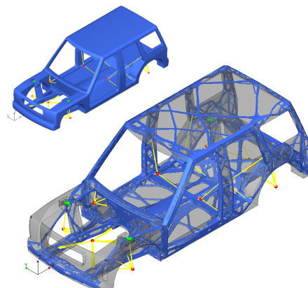
Full Body Topology Optimization
