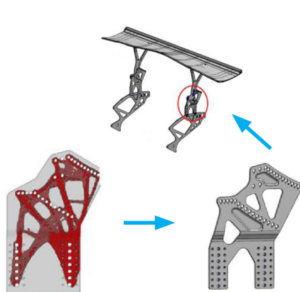
C6.R Tail Frame Assembly Courtesy of Pratt & Miller Engineering
